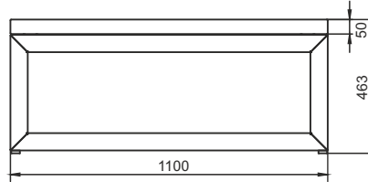
Bench 110x40x46cm
