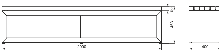
Bench 200x40x46cm
