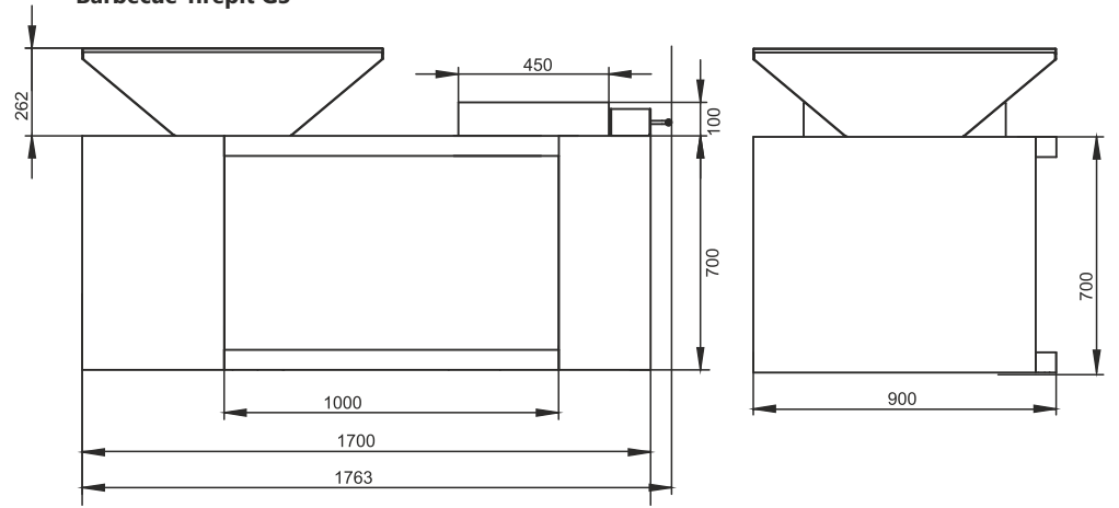
Barbecue-firepit G3
